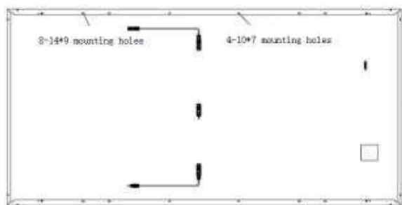
Position of mounting holes
