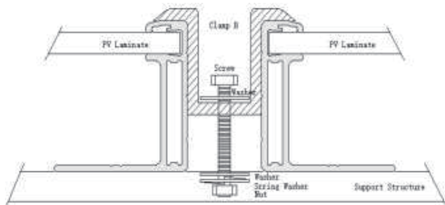
Clamp B between the modules
