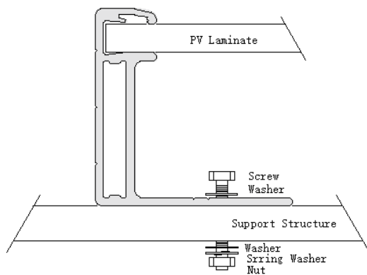
Bolt Mounting
