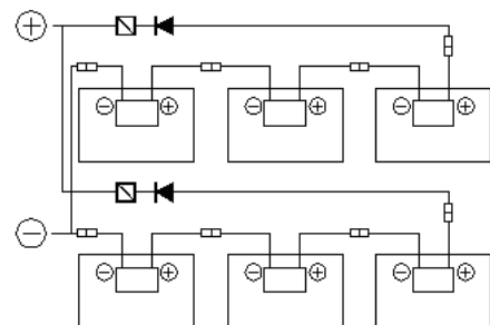
Series wiring and Parallel wiring
